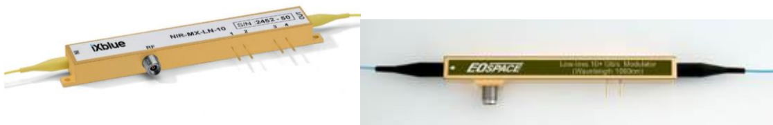
Figure 4 : Example of intensity electro-optics modulators by ixBlue (ex-Photline) (left) and EOspace (right) – (Courtesy of ixBlue/EOspace - websites)
