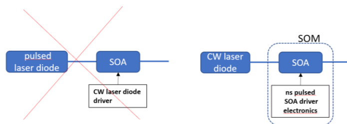
Figure 9 : SOA, when driven with specific electronics, behaves like a fiber modulator with no insertion loss (SOM)
